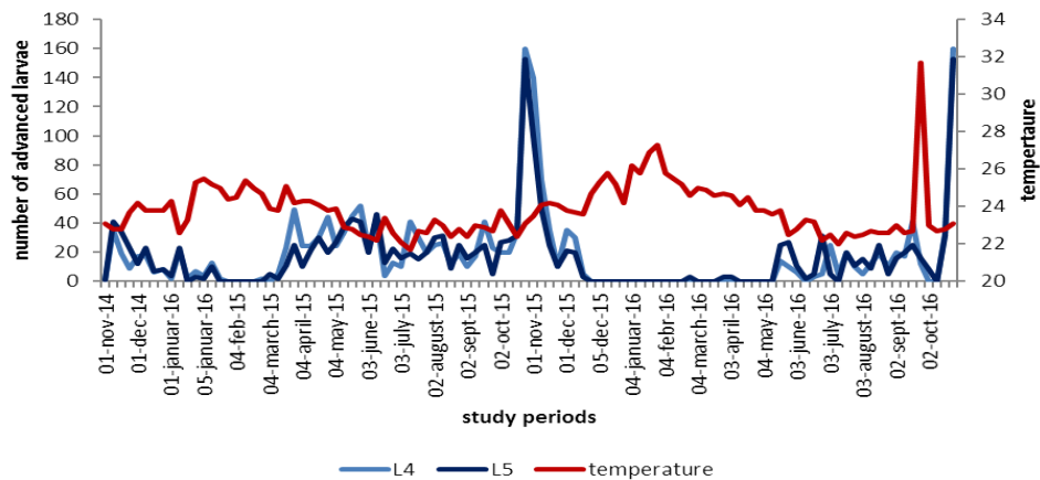
Figure 3. Numerical variation of stage IV and V larvae of Hilda cameroonensis depending on the temperature variation in a farmers plantation in Nkolfoulou (Yaoundé) from November 2014 to October 2016.
