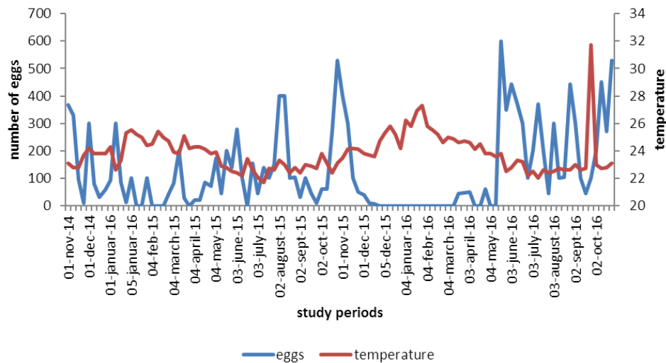
Figure 1. Numerical variation of eggs of Hilda cameroonensis depending on the temperature variation in a farmers plantation in Nkolfoulou (Yaoundé) from November 2014 to October 2016.
